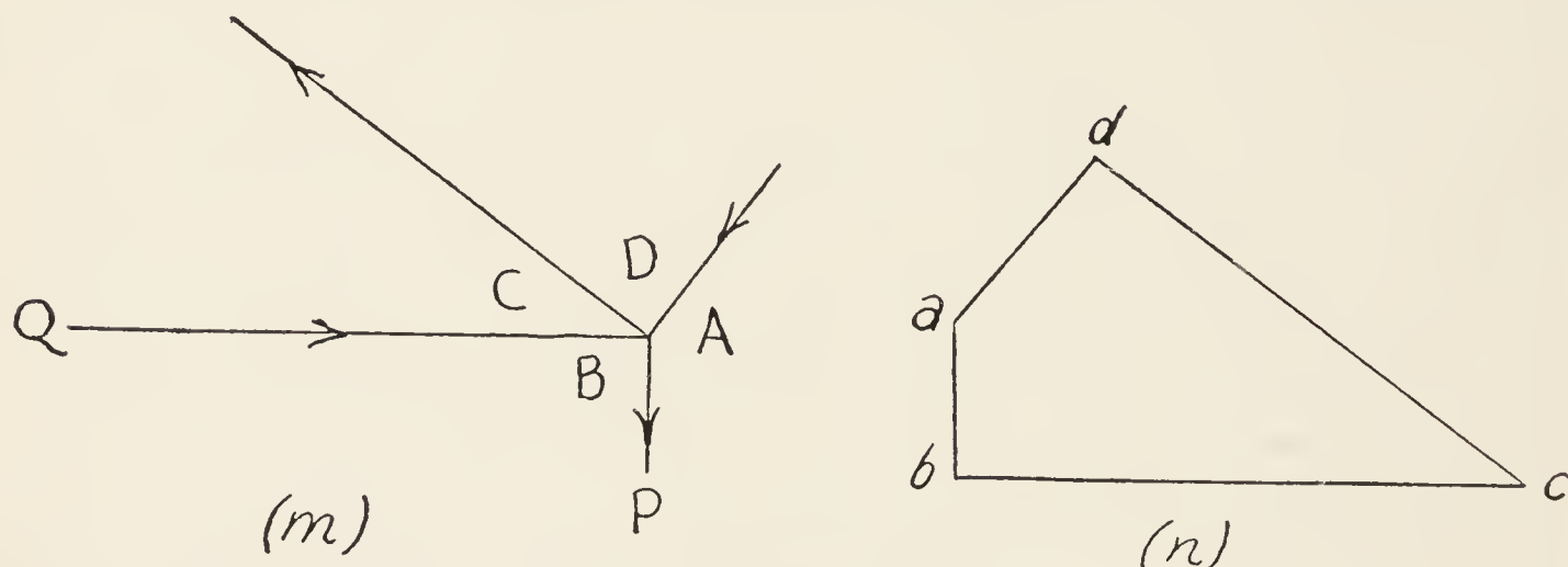
FIG. 126.—Bow's notation
