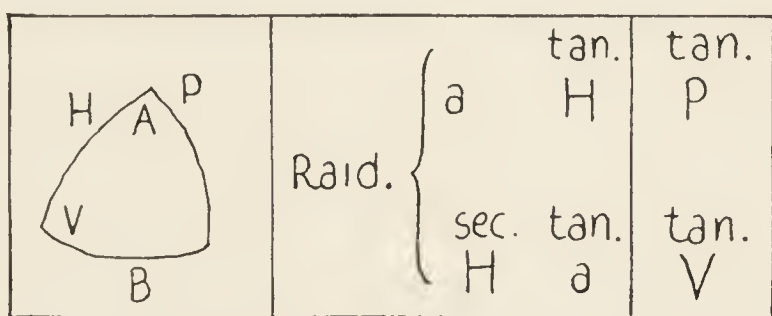
FIG. 119.—Illustrating Girard's notation in trigonometry
