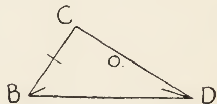
FIG. 117.—Marking the given and required parts of a triangle (1618)
