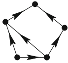
An acyclic directed graph
